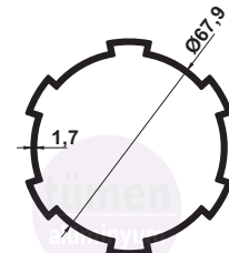
G-2926 MOTOR BORUSU 1,209 kg/m
