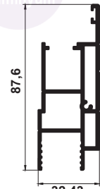
G-2916 KİLİT BAZA 1,306 kg/m
