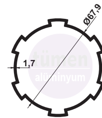
G-2926 MOTOR BORUSU 1,209 kg/m
