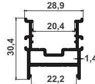
ISI-G-356 CAM DİKEY BAZA 0,467 kg/m
